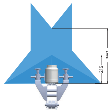
Beam geometry
